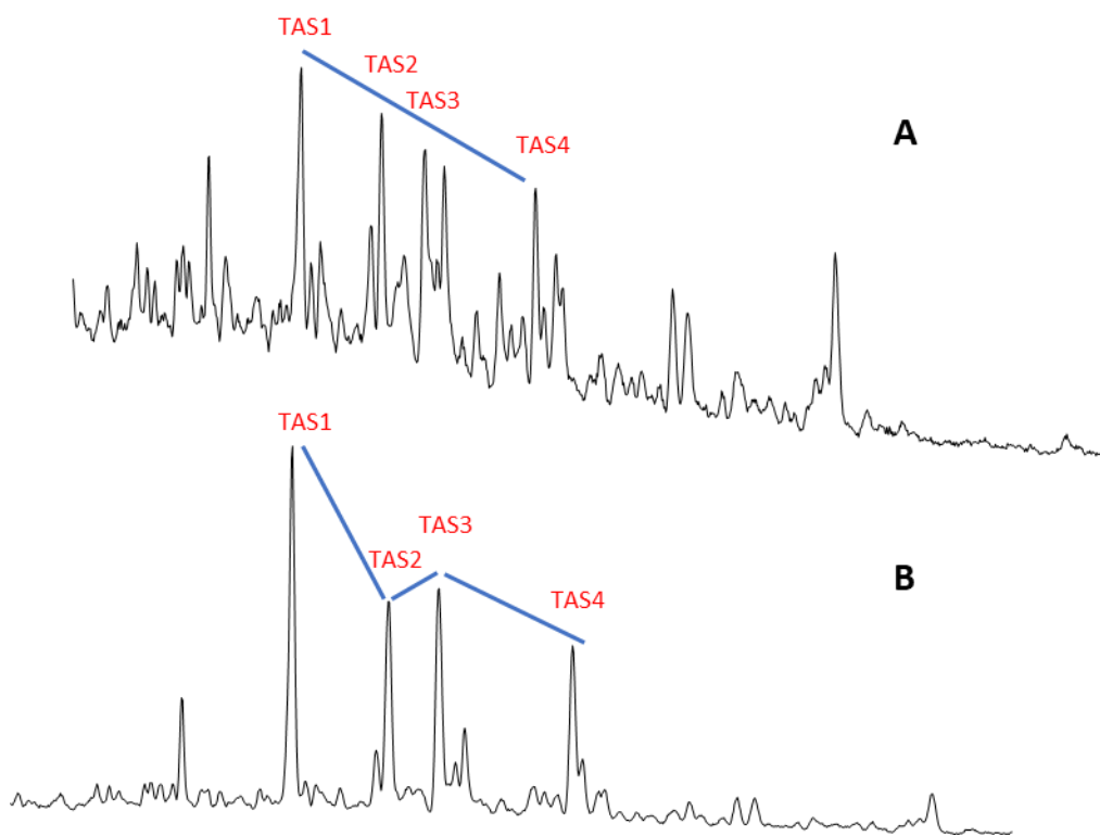
Figure 5. Biomarker m/z 231 Triaromatic Steroid Fingerprint Traces A) Ship's Tanks Composite Sample B) HC DEL 01AGO2023
