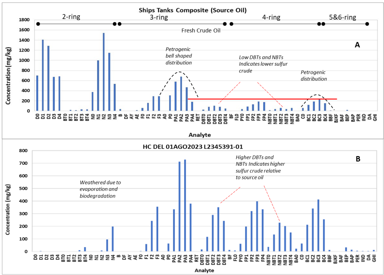
Figure 2. PAH Histograms A) Ship's Tanks Composite Sample B) HC DEL 01AGO2023
